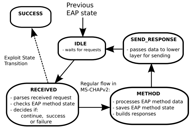
Figure 7: State flow for inner TTLS authentication with exploit on the client side. The dashed arrow indicates state transition triggered by a received EAP success after omitting the Authenticator Response in EAP-TTLS/MS-CHAPv2.
