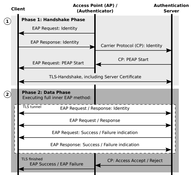
Figure 4: Sample PEAP Authentication Process
