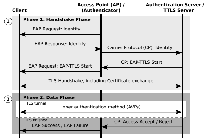
Figure 3: Sample EAP-TTLS Authentication Process
