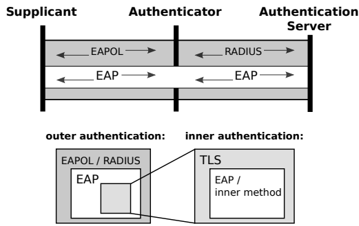
Figure 2: 802.1X Communication and Protocol Encapsulation
