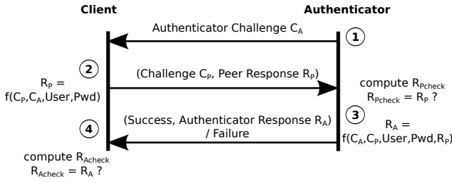
Figure 5: MSCHAPv2 Authentication Process
