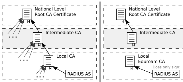
Figure 8: National certificate structure of Eduroam before and after applying countermeasure I1: On the left: Current situation with an indefinite amount of intermediate and server certificates signed by the same root CA and therefore valid for rogue authentication. On the right: Resulting structure after applying I1. Because the local Eduroam CA is only used for RADIUS AS, it is not possible anymore for an attacker to obtain a valid rogue certificate.
