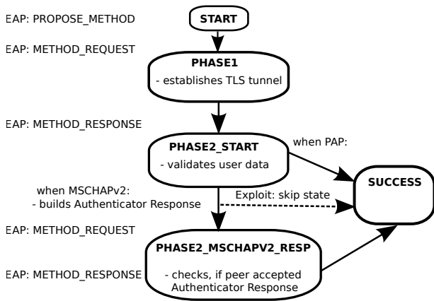
Figure 6: State flow for inner TTLS authentication on the server side. The dashed arrow indicates state skip in EAP-TTLS/MS-CHAPv2 used for the exploit.
